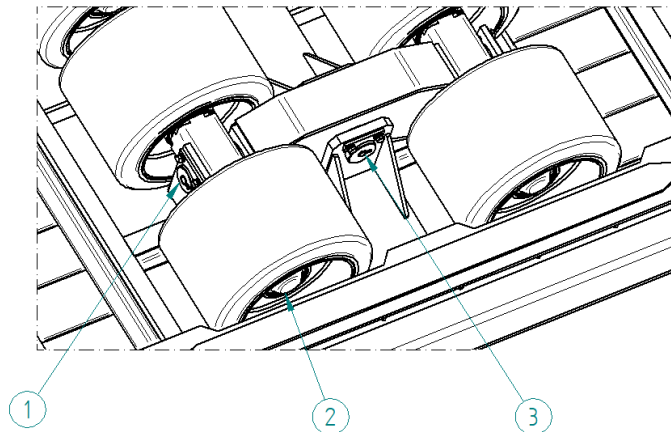
Fig. 8 Greasing points in Roll Trailer: 1) Rocker arm bolts; 2) Wheel hubs; 3) Axles bolts;
